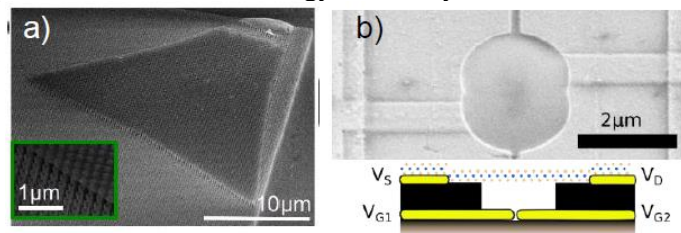
Fig. 1: a) E-beam image of suspended monolayer MoS 2 on array of nanopillars obtained at C2N. b) another geometry of suspended MoS 2 with drums geometry with integrated electrical contact. (Courtesy of J. Chaste)
